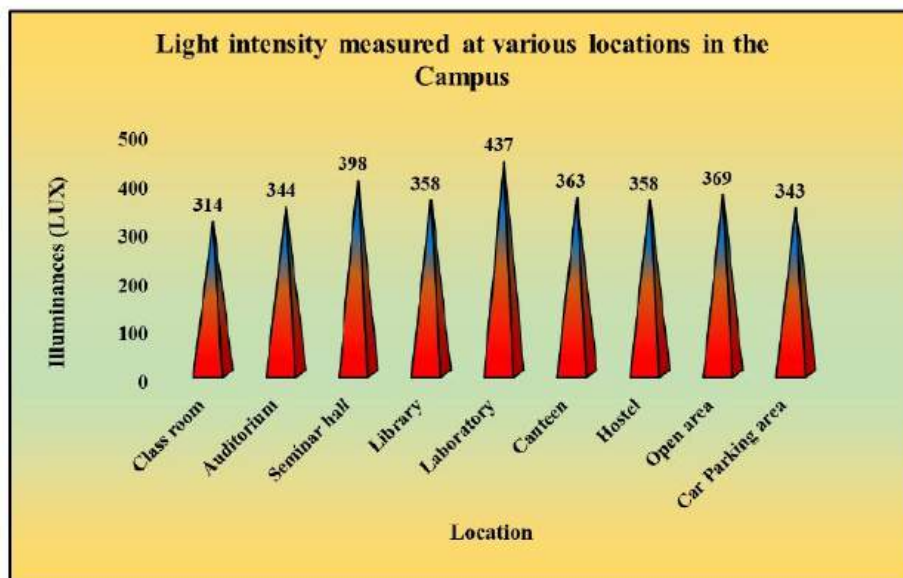
Figure 4. Light intensity Measured at the campus
